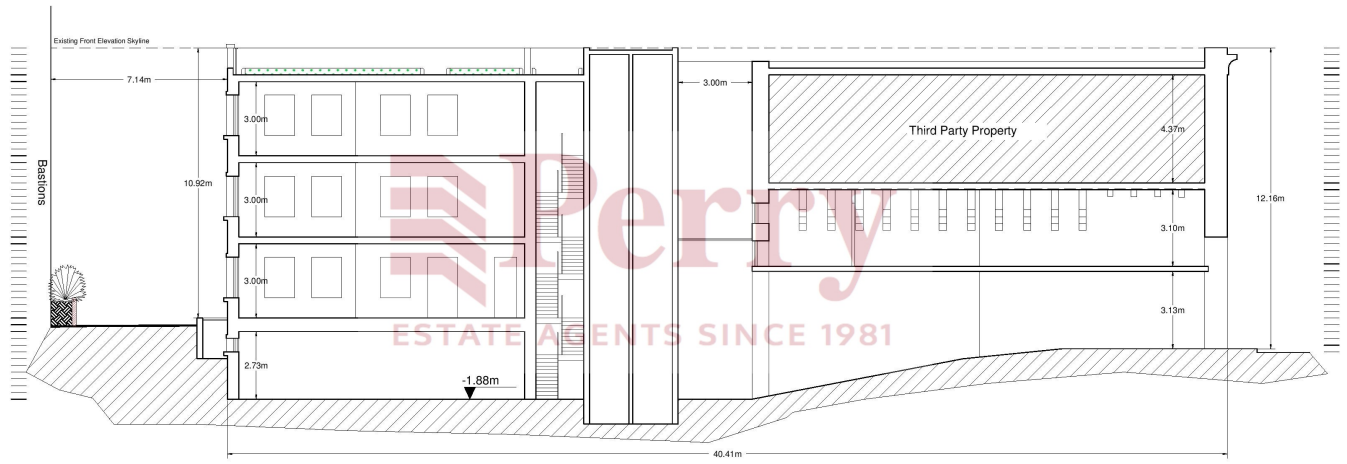
Section D - D Proposed Scale 1:100
