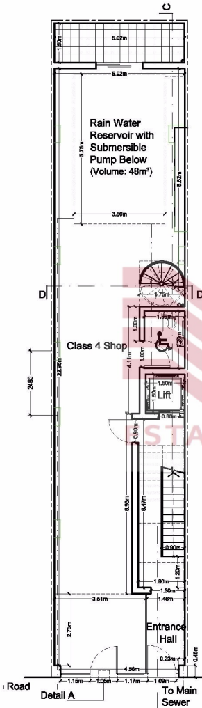
Proposed Ground Floor Plan Area: 124m² Scale 1:100
