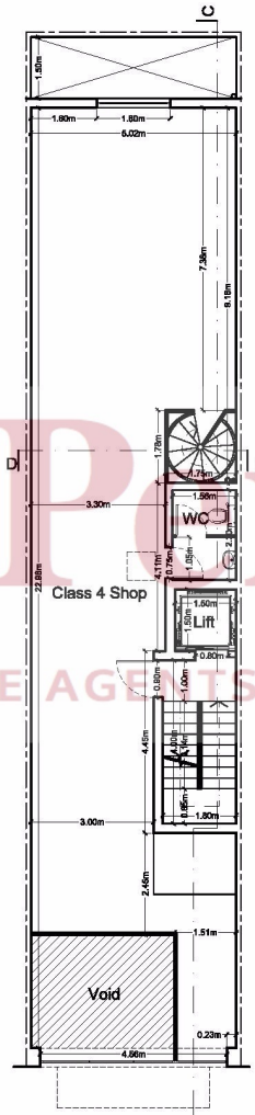
Proposed Mezzanine Floor Plan Area: 112.5m² Scale 1:100
