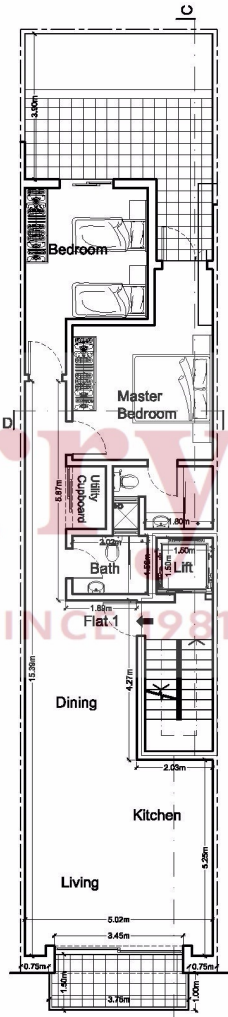
Proposed First Floor Plan Area: 106.5m²
