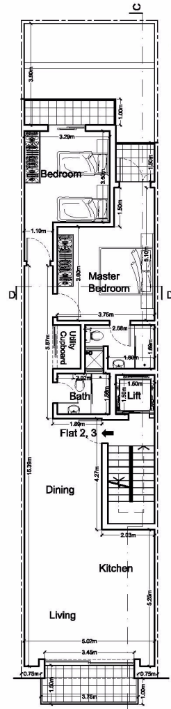
Proposed Second & Third Floor Plan Area: 106.5m²
