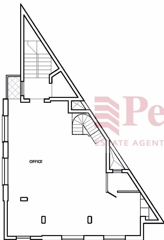
FOURTH FLOOR LEVEL SCALE 1:100 / AREA: 80sq.M.
