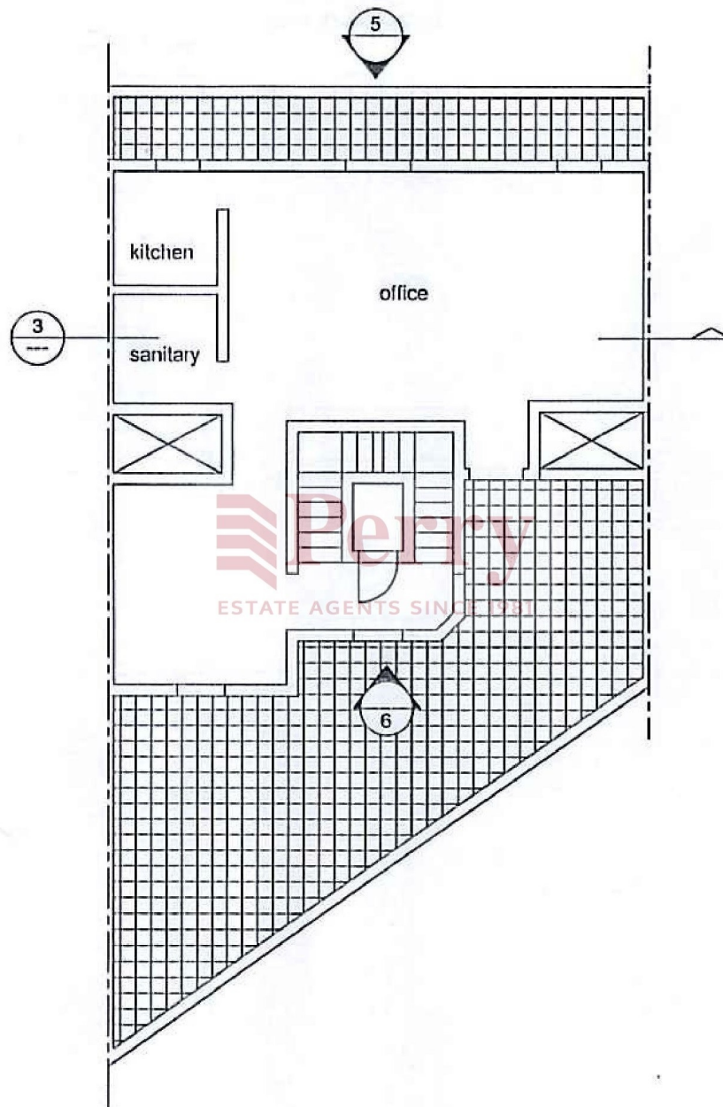
4 PROPOSED PENTHOUSE Scale 1:100
