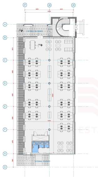
1 Office A1 - Level 0, 1 & 2 - FIT-Out - Open Plan 1:100
