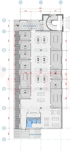
2 Office A1 - Level 0, 1 & 2 - FIT-Out - Small Cellular Office 1:100
