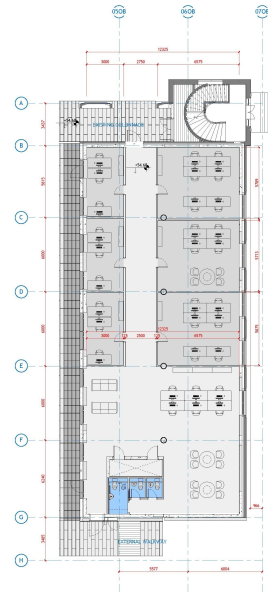
3 Office A1 - Level 0, 1 & 2 - FIT-Out - Large Cellular Office 1:100
