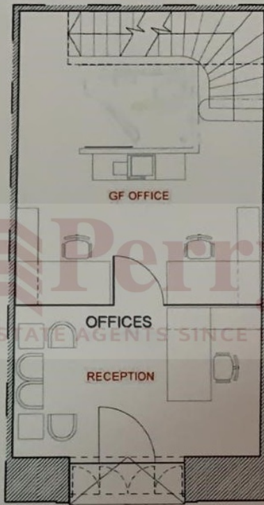
2 GROUND FLOOR SCALE 1:50
