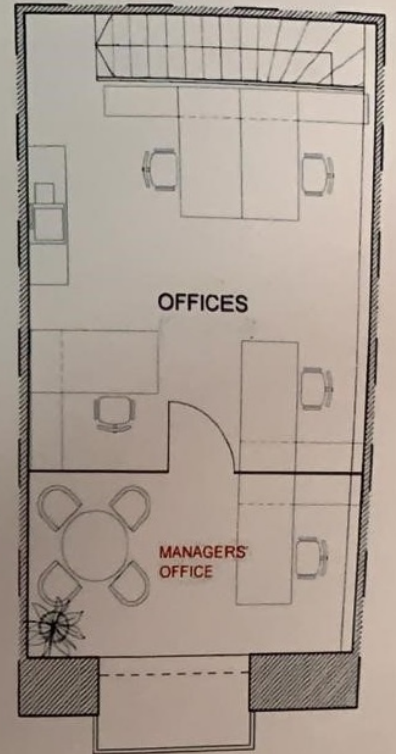
3 FIRST FLOOR SCALE 1:50
