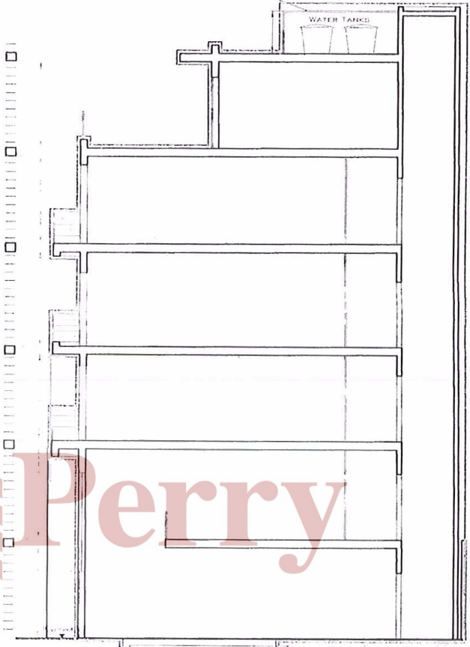
Proposed Section B-B Scale 1:100
