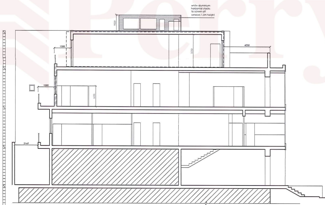
AA' Proposed Section scale 1:100
