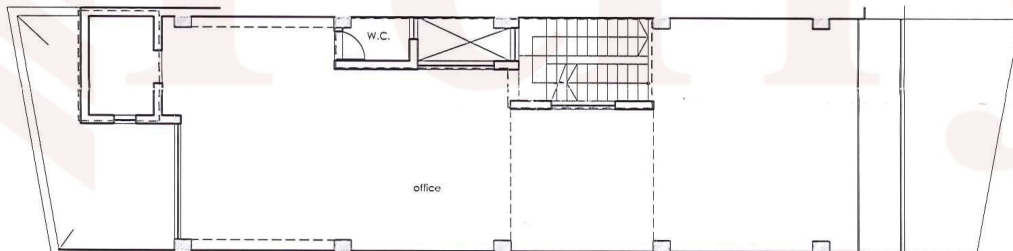
+2 Approved Second Floor scale 1:100
