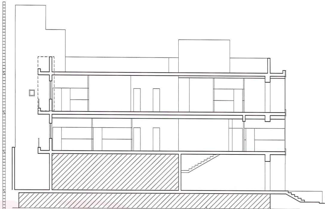
AA' Proposed Section scale 1:100
