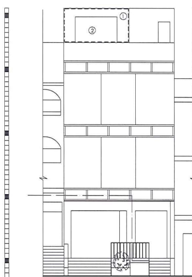
E1 Proposed Elevation scale 1:100
