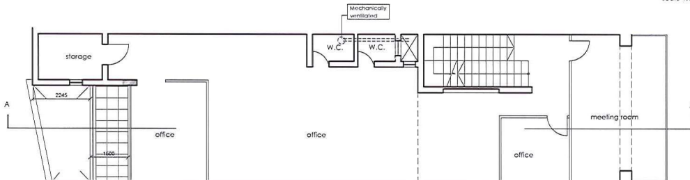
+2 Proposed Second Floor scale 1:100
