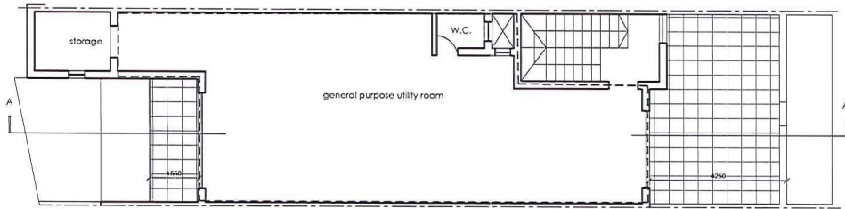
+3 Proposed Third Floor scale 1:100
