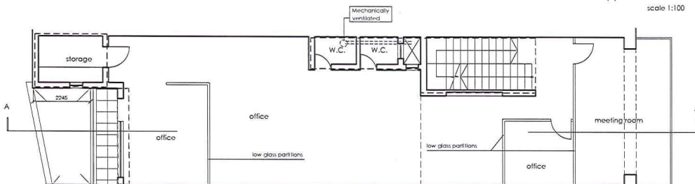
+2 Existing Second Floor scale 1:100
