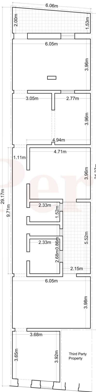
Existing Ground Floor Plan Area: 172.5m 2 Scale 1:100
