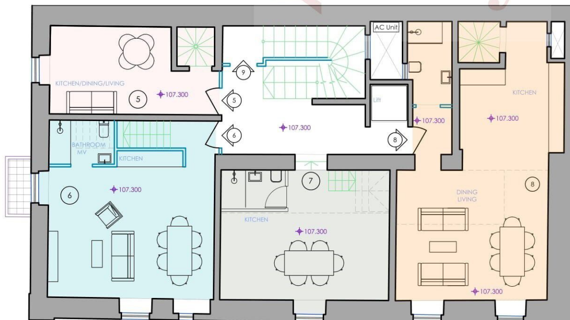
PROPOSED THIRD FLOOR
