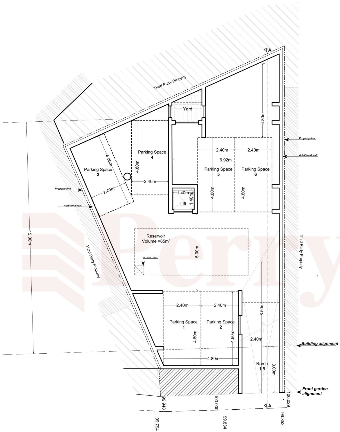
PROPOSED BASEMENT LEVEL
