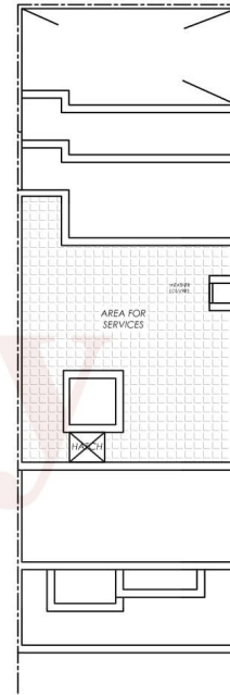
DRAWING | PROPOSED LEVEL ROOF SCALE | 1:100
