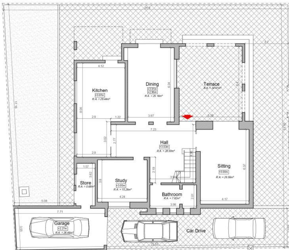
Plan at Ground Floor (Existing)
