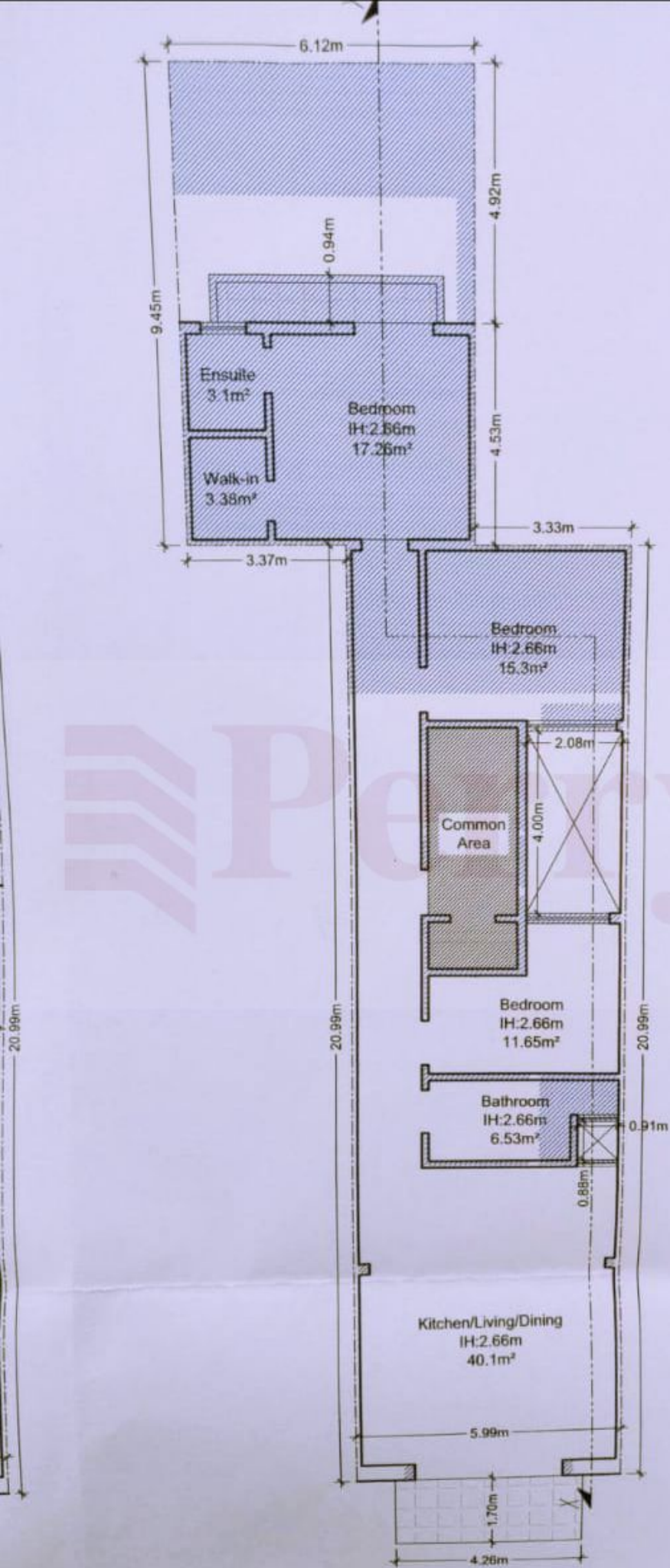
Existing Fourth Floor Plan Scale 1:100
