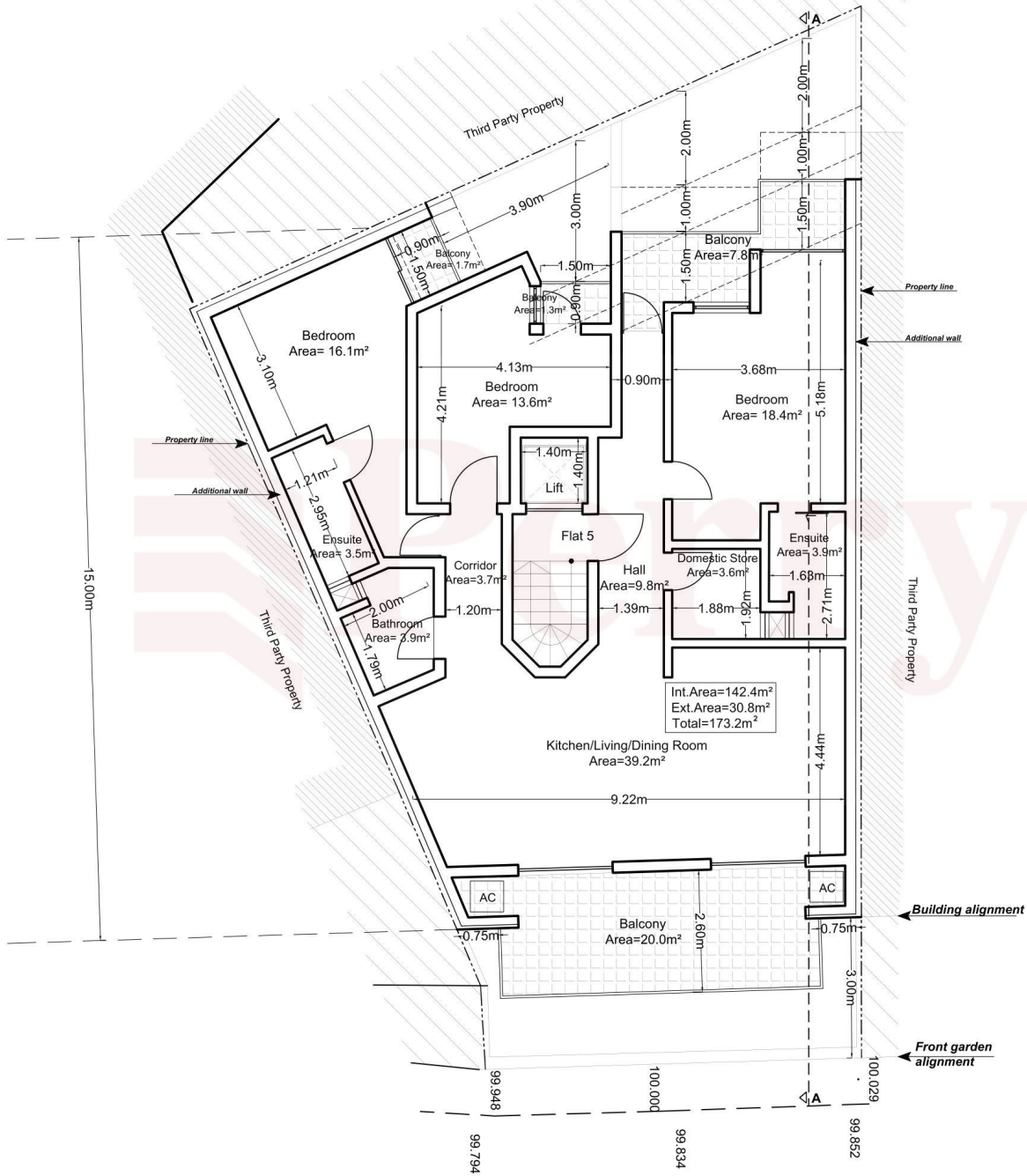
PROPOSED THIRD FLOOR
