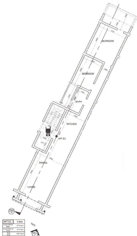
P15 PROPOSED FIRST FLOOR LEVEL SCALE 1:100
