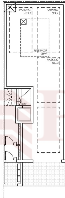
DRAWING | PROPOSED LEVEL (00) SCALE | 1:100
