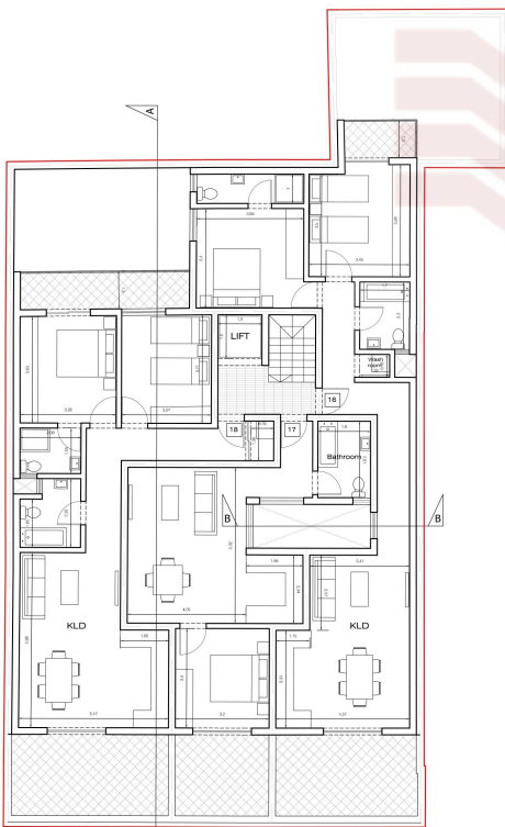
PROPOSED Level 6 Scale:- 1:100
