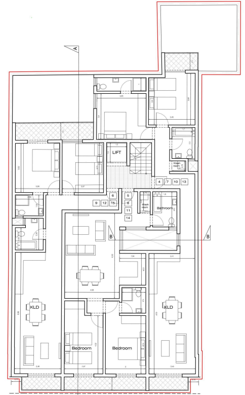
PROPOSED Levels 2-5 Scale:- 1:100
