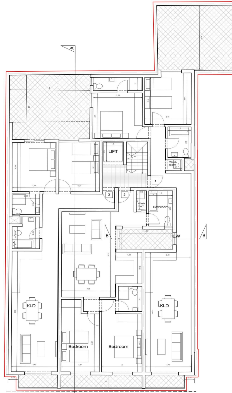
PROPOSED Level 1 Scale:- 1:100
