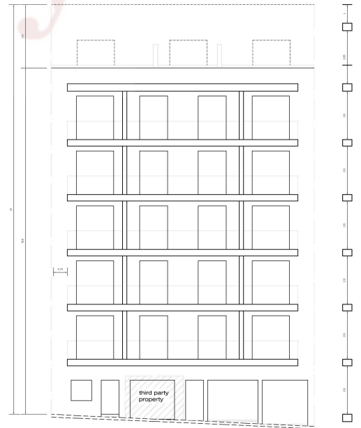
PROPOSED ELEVATION Scale:- 1:100
