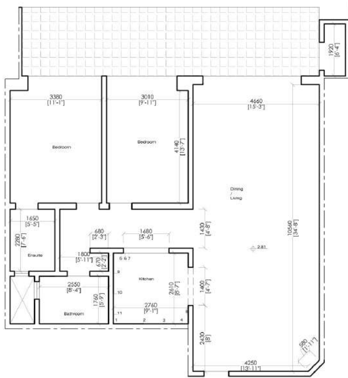
APARTMENT PLAN SCALE 1:100
