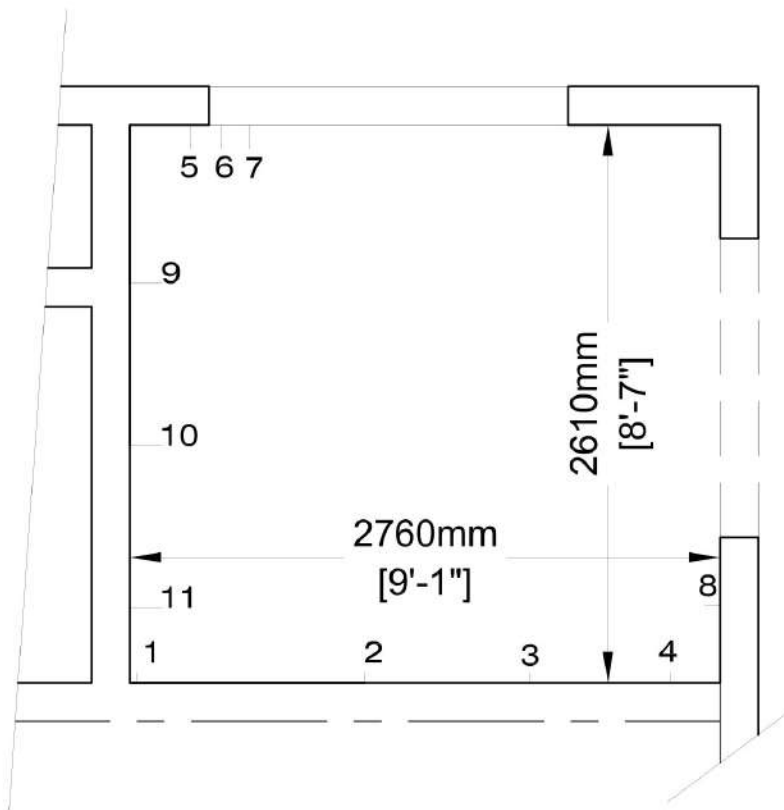
KITCHEN PLAN SCALE 1:25
