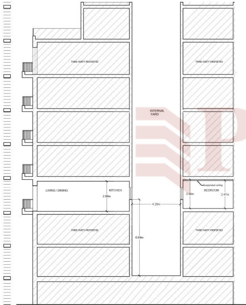
Section X-X As Existing Scale 1:100
