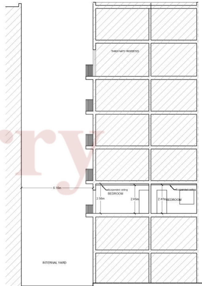
Section Y-Y As Existing Scale 1:100
