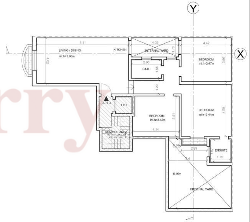
Third Floor Plan Area 117.5m 2 As Existing Scale 1:100
