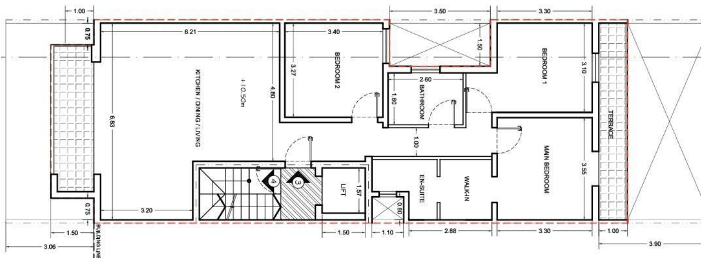
Scale 1:100
