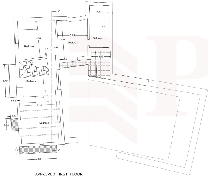
APPROVED FIRST FLOOR
