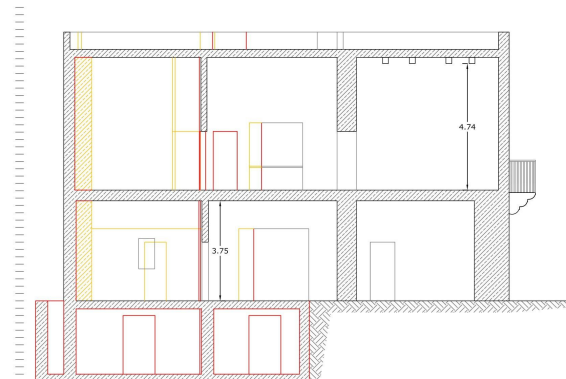
PROPOSED SECTION Y-Y
