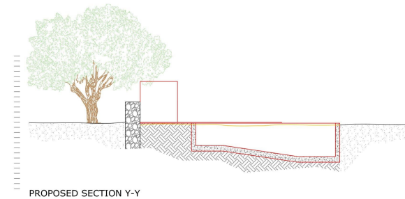
PROPOSED SECTION Y-Y
