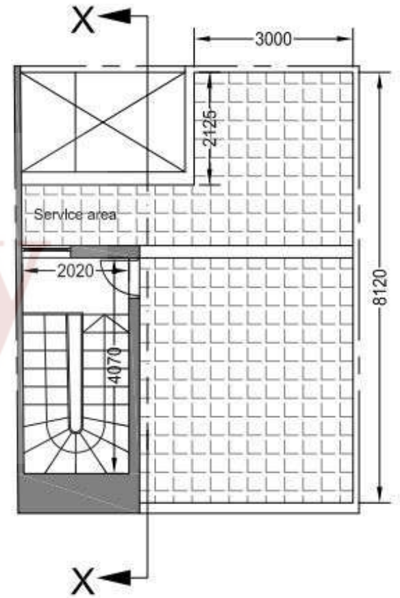
EXISTING ROOF
