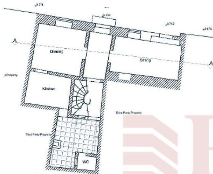
EXISTING GROUND FLOOR PLAN (pre 1967) scale 1:100
