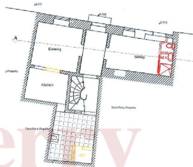
PROPOSED GROUND FLOOR SHOWING ALTERATIONS scale 1:100
