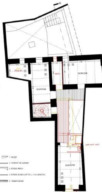
02. FIRST FLOOR PLAN - AS PROPOSED
