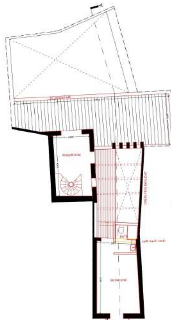
03. SECOND FLOOR PLAN - AS PROPOSED
