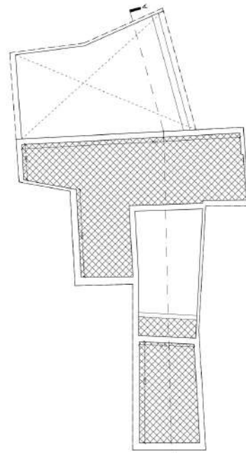
03. UPPER ROOF PLAN - AS EXISTING (PRE-1967 WITH CHANGES)
