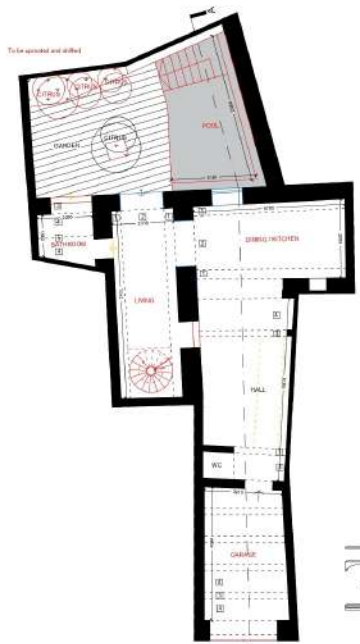
01. GROUND FLOOR PLAN - AS PROPOSED SITE EXTENTS ± c. 151.8sq. m
