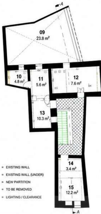
02. FIRST FLOOR PLAN - AS EXISTING (PROPOSED WITH CONVENIENCE)
