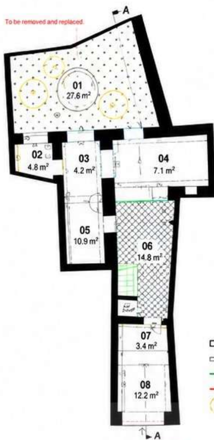
01. GROUND FLOOR PLAN - AS EXISTING (PROPOSED WITH CONVENIENCE)
