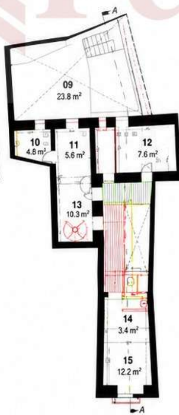
05. FIRST FLOOR PLAN - AS PROPOSED
