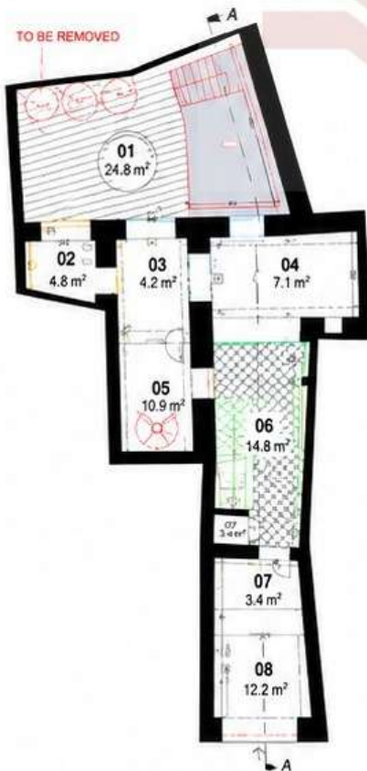
04. GROUND FLOOR PLAN - AS PROPOSED (SITE AREA 112.6 m 2 / BUILT AREA 66.5 m 2 )
