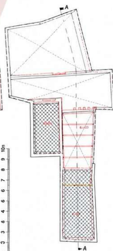
07. UPPER ROOF PLAN - AS PROPOSED
