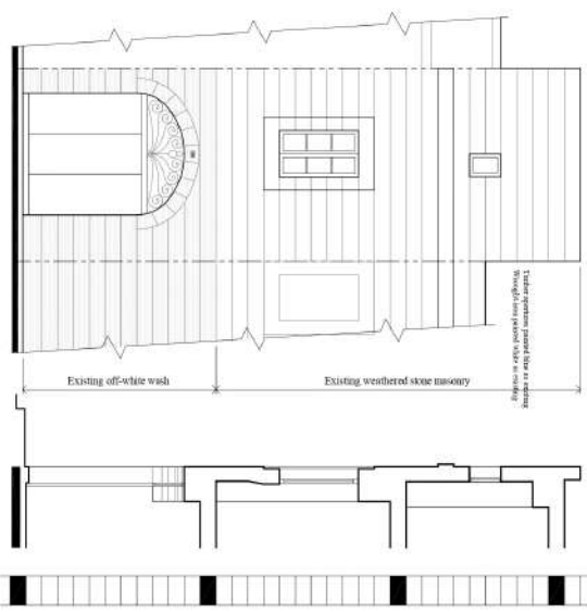
FACADE (to be retained) Scale 1:50
