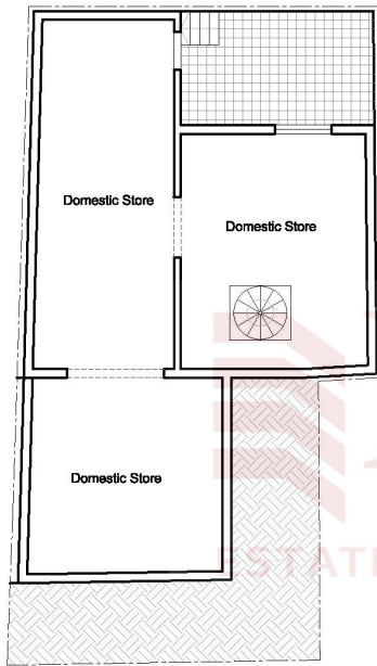
Basement Level (as existing) Scale 1:100
