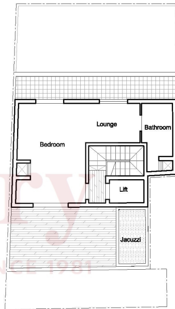
Sixth Floor Level (as proposed) Scale 1:100
