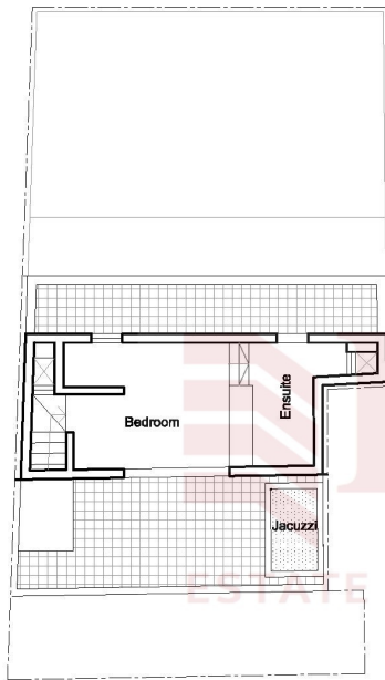
Fifth Floor Level (as existing) Scale 1:100
