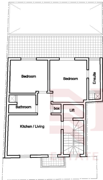
Second Floor Level (as existing) Scale 1:100
