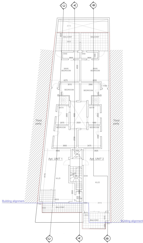
EXISTING FIRST FLOOR PLAN AS APPROVED IN PA
