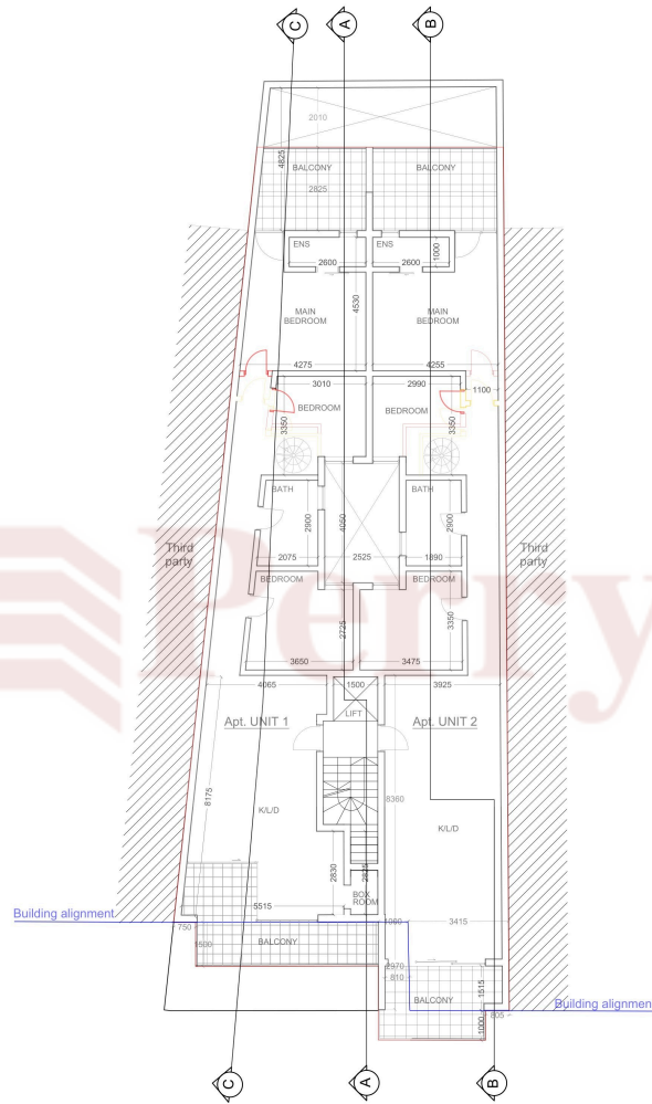
SUPERIMPOSED FIRST FLOOR PLAN
