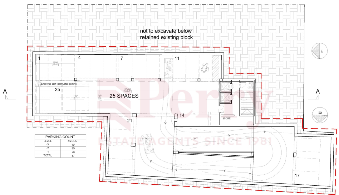
Proposed Basement -2 Scale 1:100
