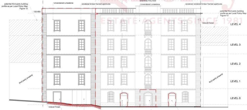
Proposed Elevation 1
