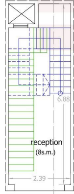
existing ground floor
