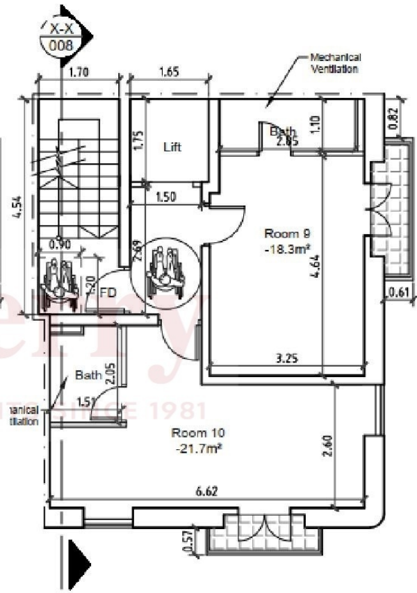
03 FIFTH FLOOR PLAN PLAN_AS PROPOSED SCALE 1:100
