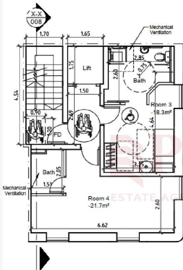
03 SECOND FLOOR PLAN PLAN_AS PROPOSED SCALE 1:100
