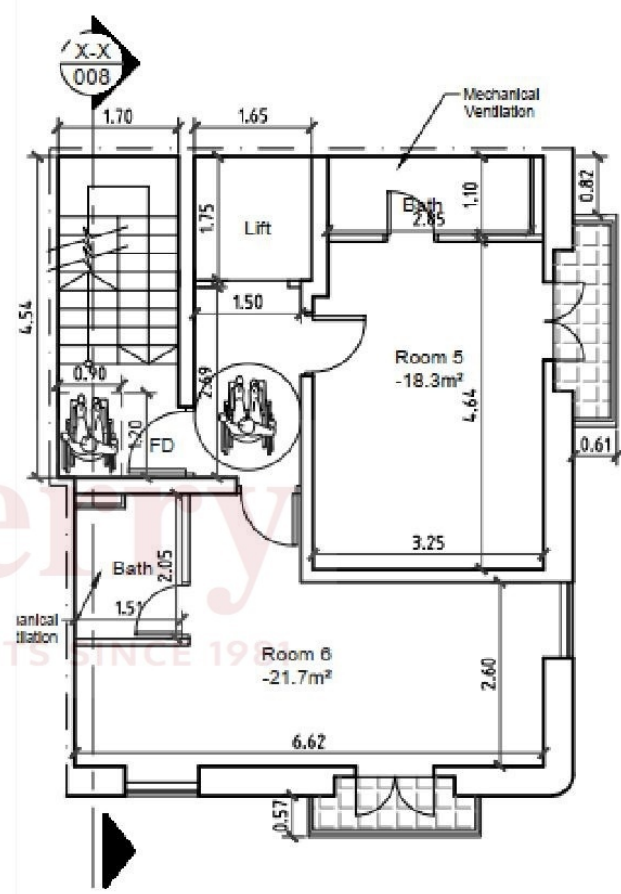
03 THIRD FLOOR PLAN PLAN_AS PROPOSED SCALE 1:100
