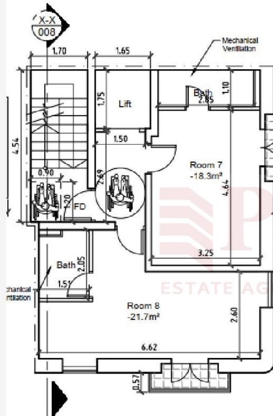
03 FOURTH FLOOR PLAN PLAN_AS PROPOSED SCALE 1:100
