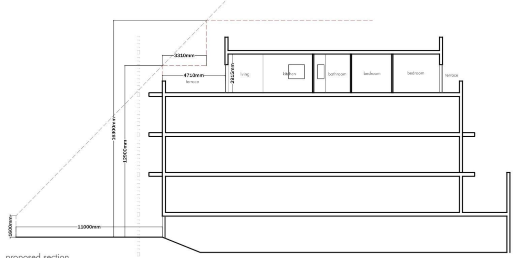
PROPOSED SECTION SCALE 1:100
