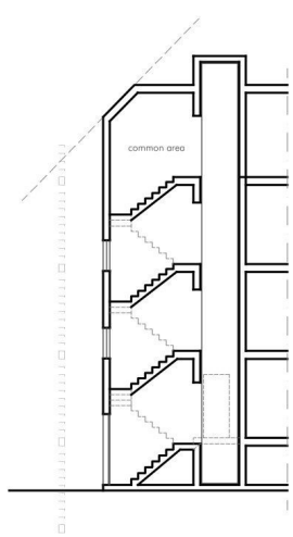
PROPOSED SECTION THROUGH COMMON AREA SCALE 1:200
