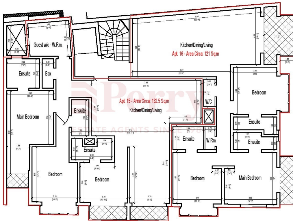
Sixth Floor Plan
