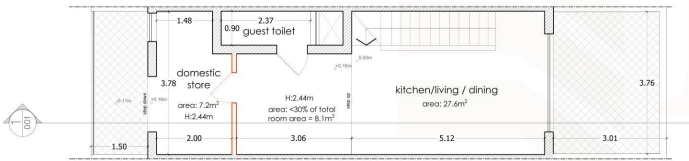
2 PROPOSED PLAN AT RECEDED FLOOR SCALE 1:100
