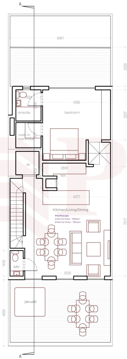
PROPOSED LEVEL 3 (PENTHOUSE) Scale:- 1:100 - CLEAN COPY
