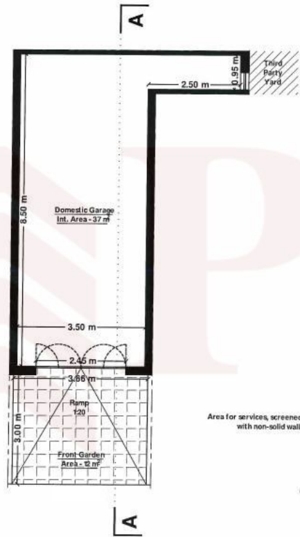
A01 EXISTING GROUND FLOOR PLAN 01 SCALE 1:50
