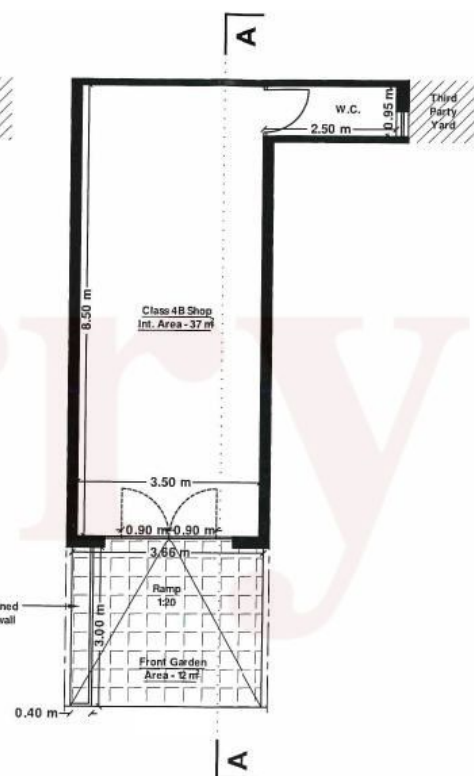
A03 PROPOSED GROUND FLOOR PLAN 03 SCALE 1:50
