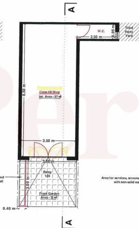
A02 EXISTING/PROPOSED GROUND FLOOR PLAN 02 SCALE 1:50
