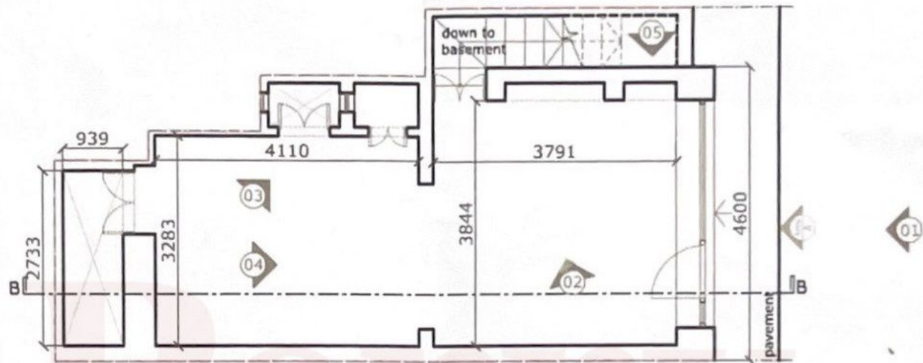
PLAN - LEVEL 0 GROUND FLOOR
