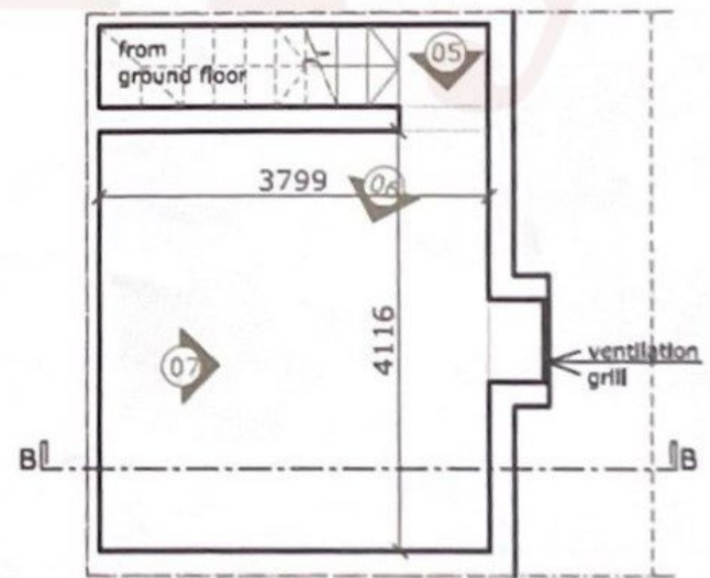
PLAN - LEVEL -1 BASEMENT
