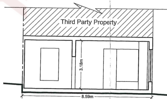
S2 D2 PROPOSED TRANSVERSE SECTION B-B Scale 1:100
