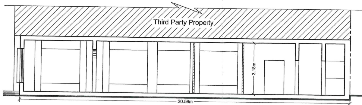
S1 D2 PROPOSED LONGITUDINAL SECTION A-A Scale 1:100
