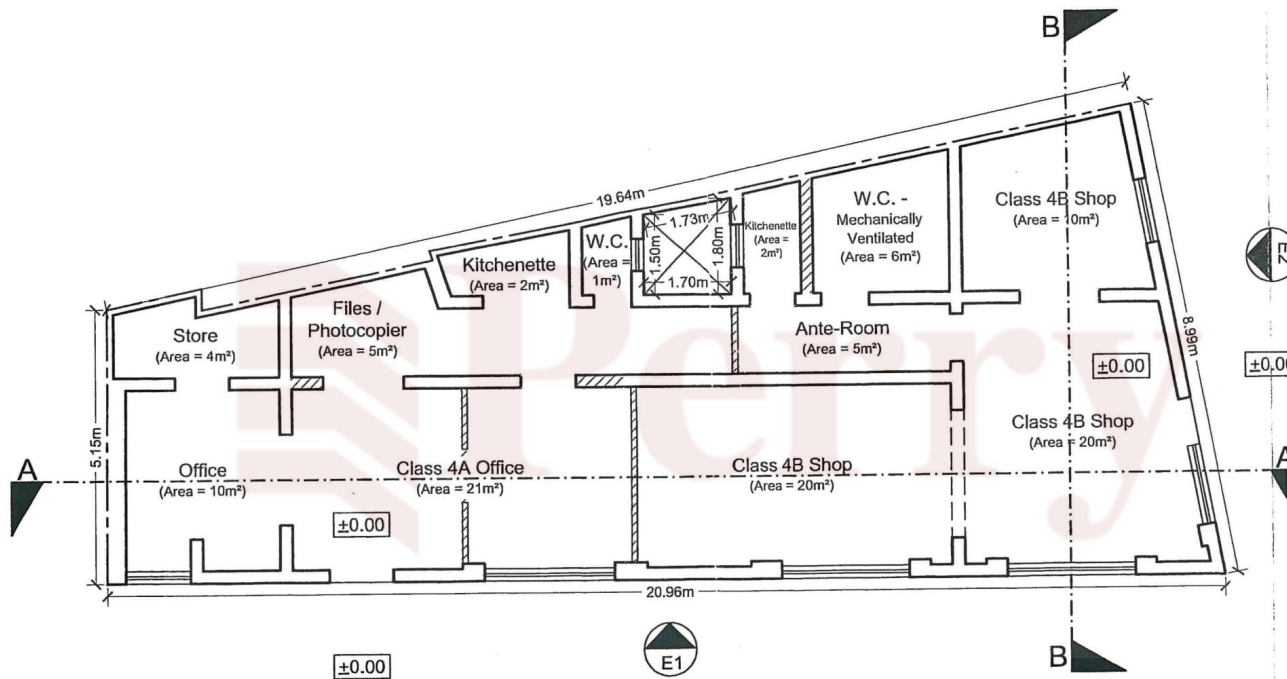
P1 PROPOSED GROUND FLOOR PLAN D1 Floor Area = 137m 2 Scale 1:100
