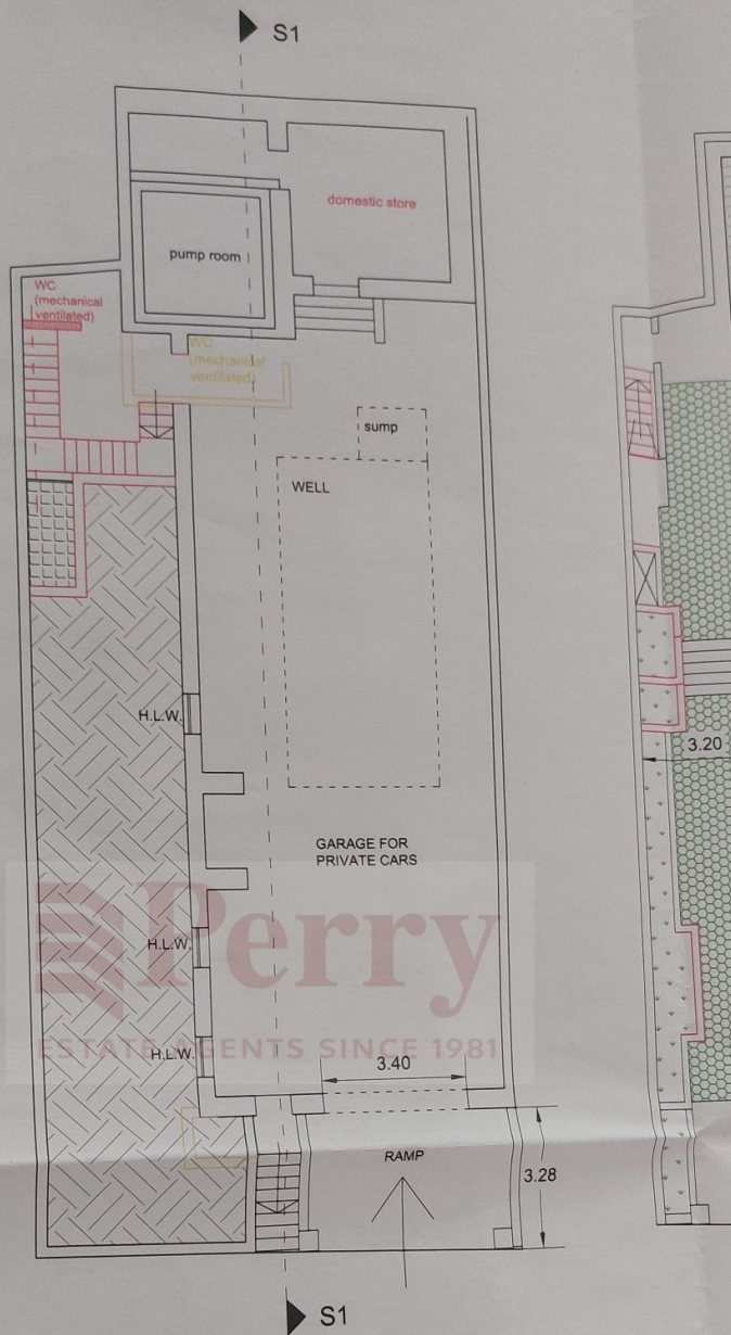
PROPOSED BASEMENT PLAN
