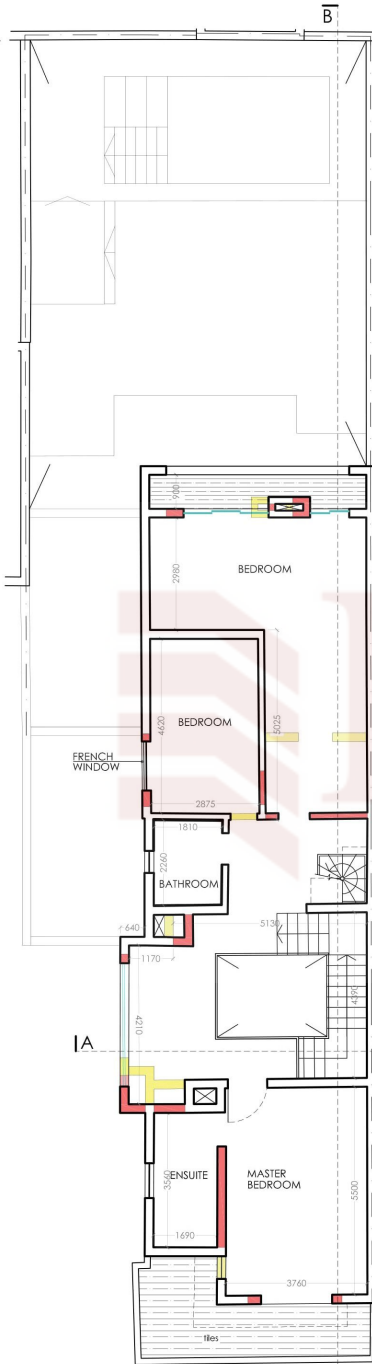
FIRST FLOOR SCALE 1:100 AREA: 127.6m 2
