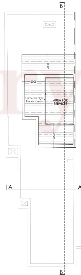
ROOF SERVICE PLAN SCALE 1:100
