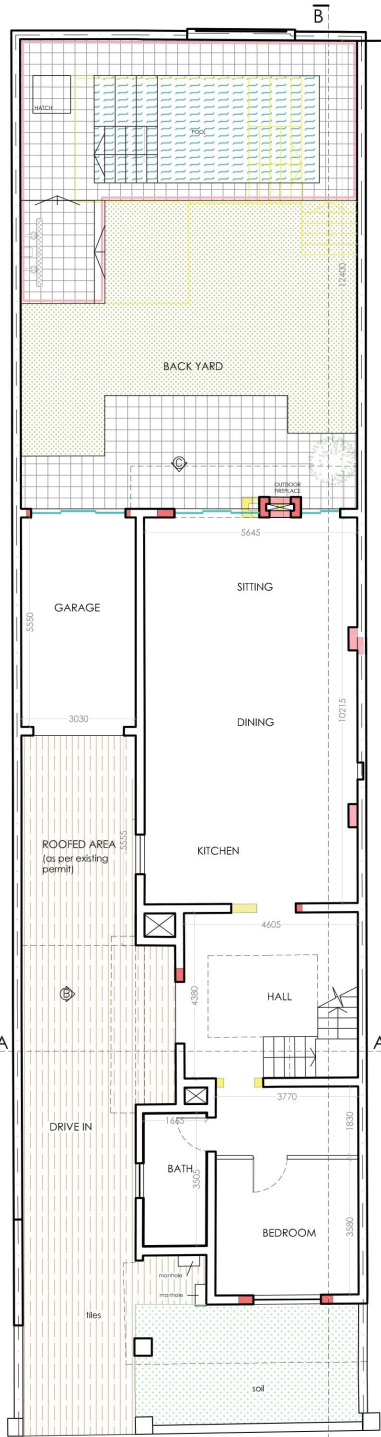
GROUND FLOOR SCALE 1:100 AREA: 123.9m 2
