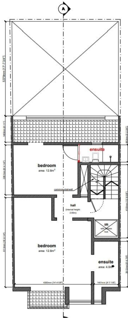
As Proposed Fifth Floor Level Plan scale 1:100
