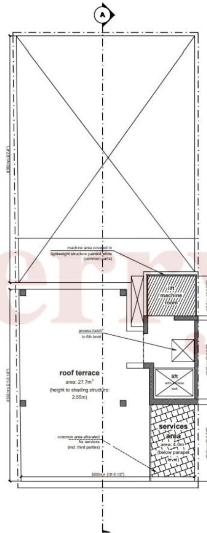
As Proposed (No Changes) Roof Level Plan scale 1:100
