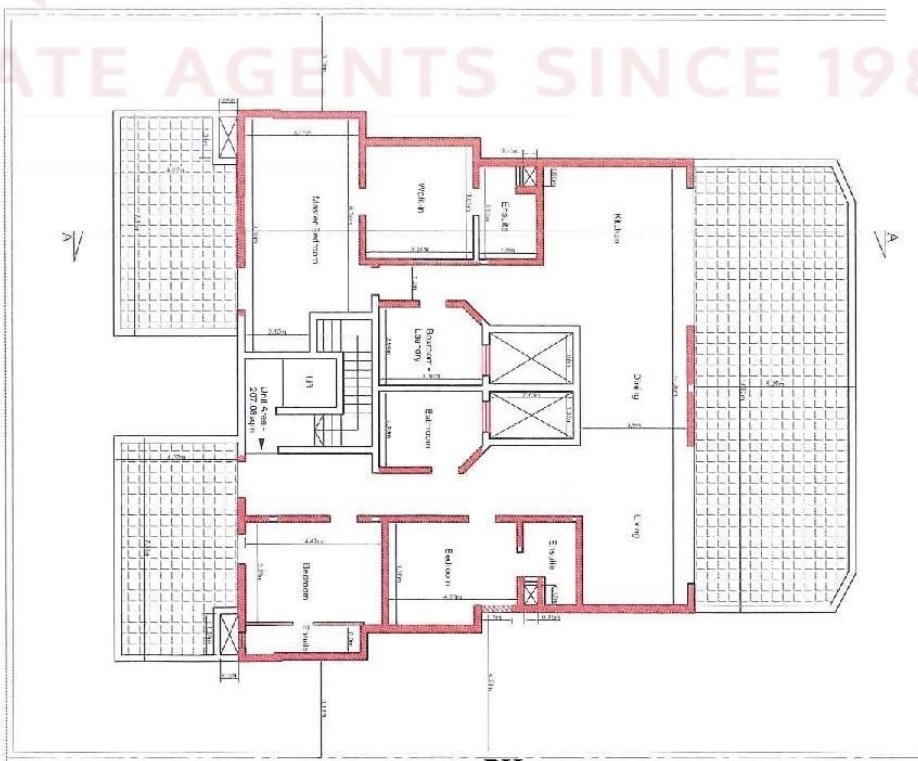
PROPOSED LEVEL 5 PLAN UNIT AREA (INTERNAL) - 207.08SQM
