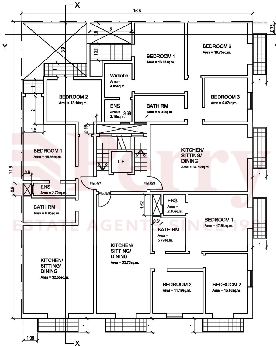
SECOND & THIRD FLOOR PLAN Built up Area = 328.61sq.m.
