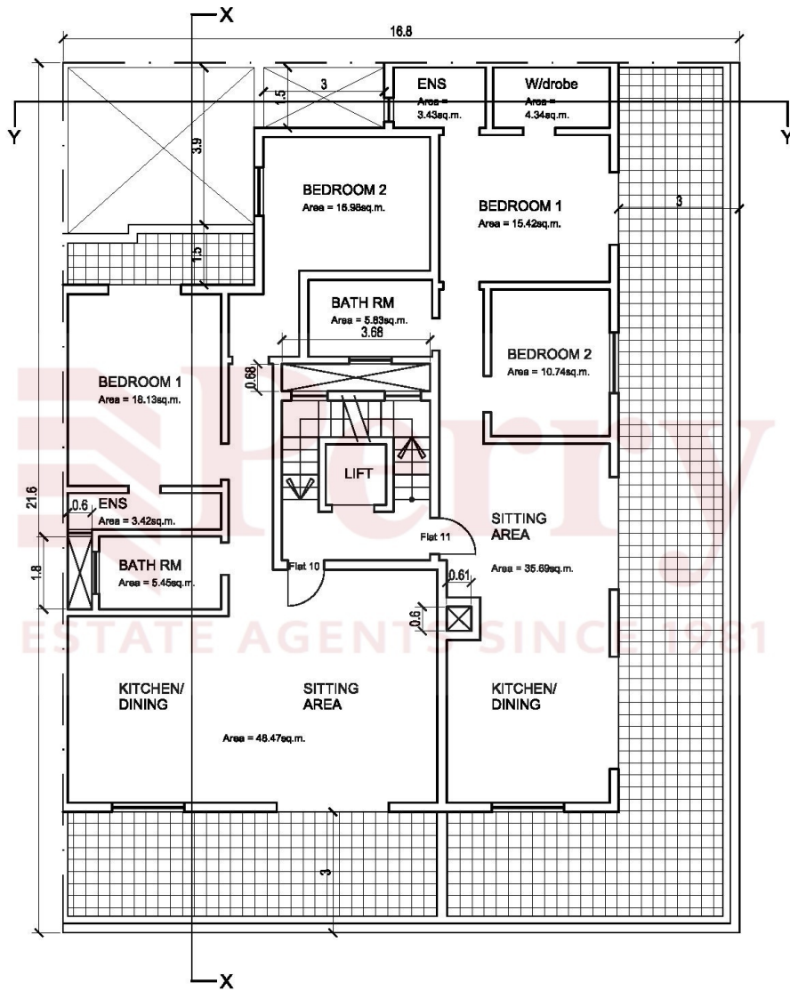
RECEDED FLOOR PLAN Built up Area = 221.13sq.m.
