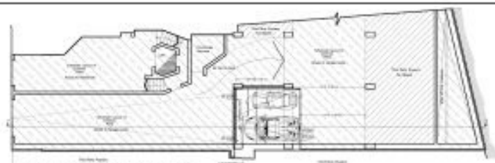
Existing Plan of Interconnected Garage Level - Level 8
