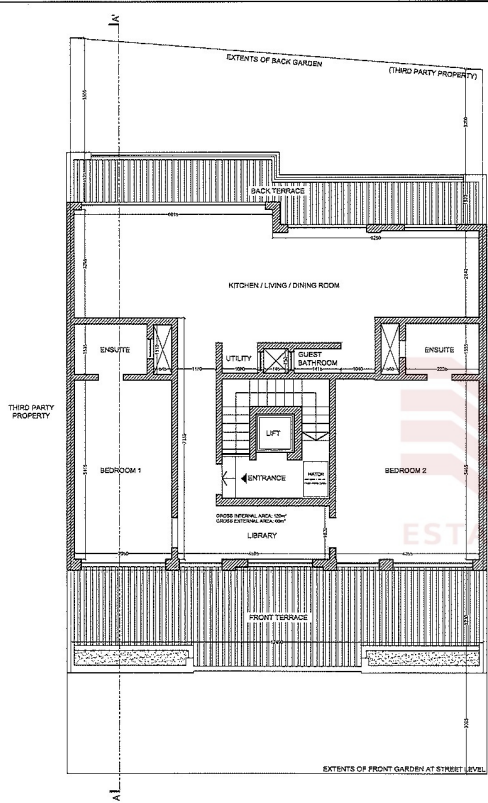
EXISTING THIRD FLOOR PLAN SCALE 1:100
