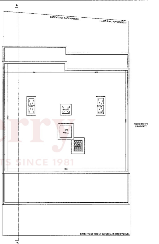
EXISTING FOURTH FLOOR PLAN SCALE 1:100
